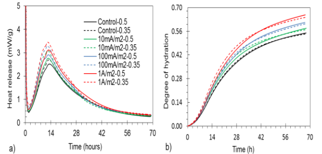
Figure 3. Heat released (a) and degree of hydration (b) as function of time for cement paste with w/c 0.5 and 0.35.
