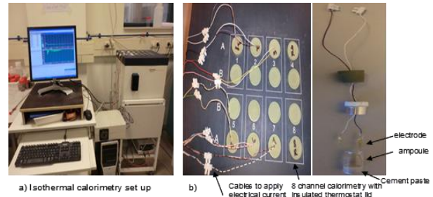
Figure 2. (a) Isothermal calorimeter (TAM-Air-314) used to measure heat release of cement paste; (b) Schematic pictures of the holders for “under current” regime (Series C).
