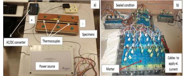
Figure 1. Experimental set-up for measurements of temperature increase in cement paste and mortar specimens due to electrical current flow (Series A) (a) and experimental set up of electrical current flow through mortar specimens in sealed condition (Series B) (b).
