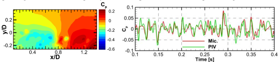
Fig. 5. Example of instantaneous PIV-based pressure field (left) and comparison to microphone signal (right)
