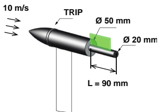
Fig. 1. Wind-tunnel model
