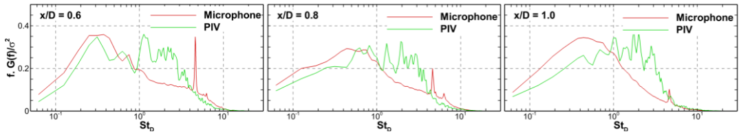
Fig. 7. Estimated normalised power spectral density of microphone and PIV pressure signals
