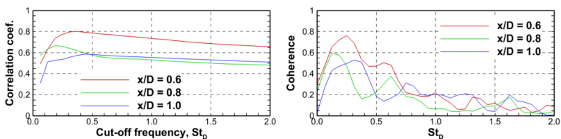
Fig. 6. Normalised cross-correlation coefficient between PIV and microphone pressure signal (left) and coherence (right)
