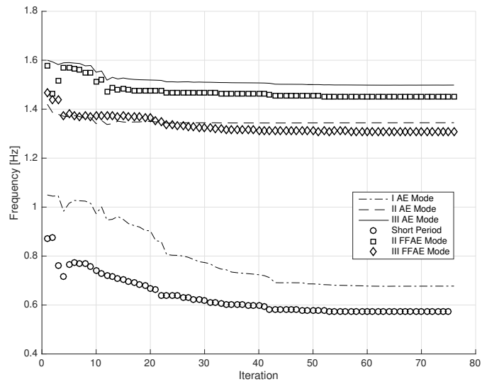
Fig. 9 History of modal frequencies during aeroelastic tailoring optimization. AE : Aeroelastic, FFAE: Free-flying Aeroelasticity.
