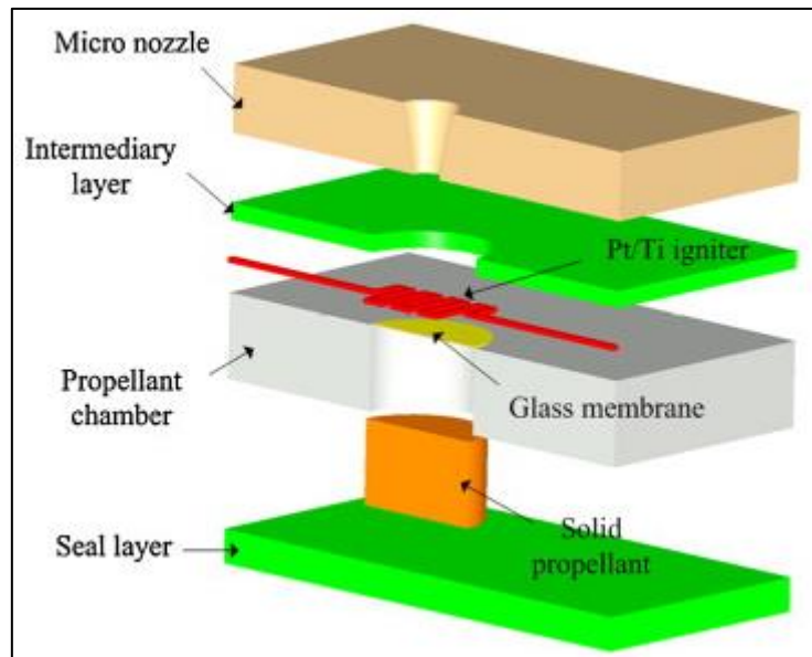
6 7 Figure 4 – Example of a solid propellant micro-thruster (adapted from [60]). 8
