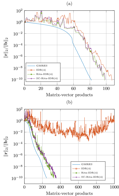
Figure 2: ( Example 2 ) Evolution of the residual norm of full GMRES, IDR(4), Ritz-IDR(4), and SC-Ritz-IDR(4). (a) Diffusion-dominated example. (b) Convection-dominated example.
