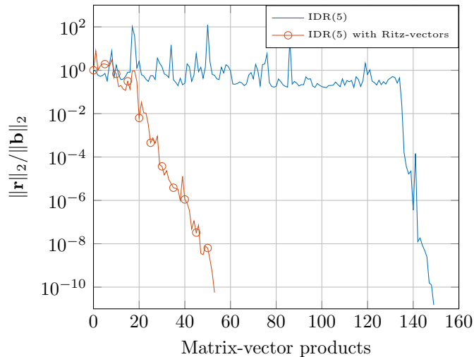
Figure 6: ( Example 6 ) Evolution of the residual norm of full IDR(5) and IDR(5) with recycling with the four eigenvectors associated with the smallest magnitude eigenvalues of the matrix (29).
