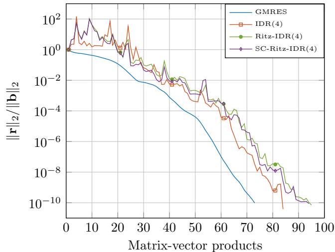
Figure 4: ( Example 4 ) Evolution of the residual norm of full GMRES, IDR(4), Ritz-IDR(4), and SC-Ritz-IDR(4) for the matrix Sherman5 using ILU preconditioner.
