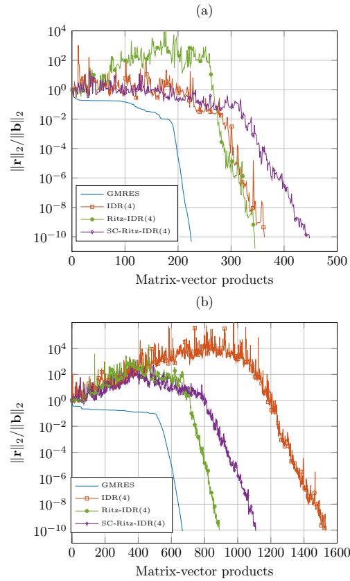
Figure 1: ( Example 1 ) Evolution of the residual norm of full GMRES, IDR(4), Ritz-IDR(4), and SC-Ritz-IDR(4). (a) Diffusion-dominated example. (b) Convection-dominated example.
