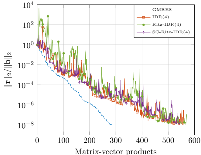
Figure 5: ( Example 5 ) Evolution of the residual norm of full GMRES, IDR(4), Ritz-IDR(4), and SC-Ritz-IDR(4) for the matrix ADD20.
