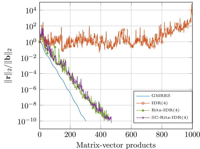
Figure 3: ( Example 3 ) Evolution of the residual norm of full GMRES, IDR(4), Ritz-IDR(4), and SC-Ritz-IDR(4).
