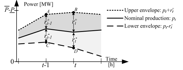
Fig. 4: Unit's operating range for power capacity
