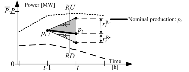
Fig. 5: Unit's operating range for ramp capability
