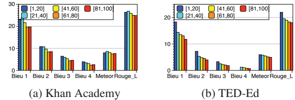
Figure 2: Results of question generation with different source sentence lengths..
