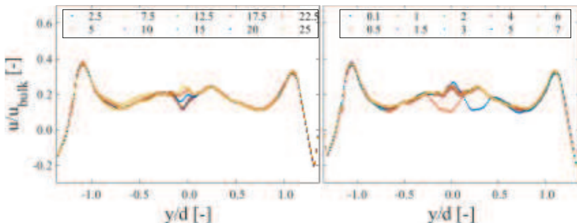
Fig. 10 Velocity profiles at x/d = 2 , where the sampling frequency is at 7.26Hz and the sample size is at 315 snapshots. On the left change in amplitude from 2.5% to 25% of mean with the frequency at 1 Hz. On the right change in frequency from 0.1 – 7 Hz with amplitude 25% of mean.
