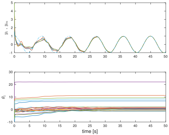
Fig. 4. Synchronization of the outputs of each agent i to the leader reference output, and adaptive gains.
