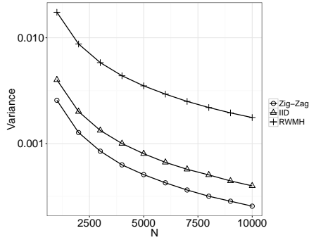
(a) Variance for f(x) = x .
