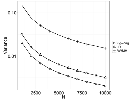
(b) Corresponding plot for f(x) = x^2 .
