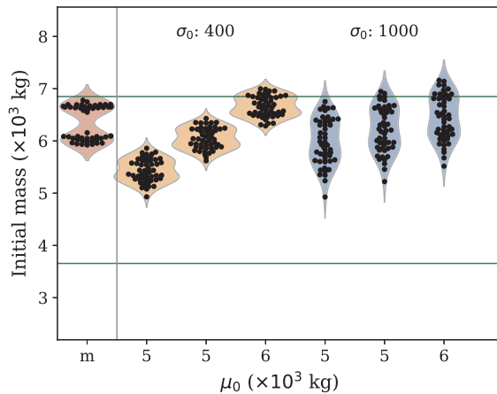
Fig. 14. Prior test in relation with the true mass data. Green horizontal lines refer to m_{oew} and m_{mtow} . \sigma_0 grouped by different colors. (For interpretation of the references to colour in this figure legend, the reader is referred to the web version of this article.)
