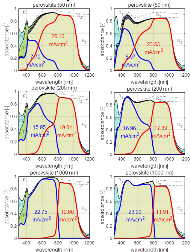
Fig. 5: Absorbance versus wavelength for every layer in the standard three-terminal perovskite / silicon tandem. White area indicates reflection losses. Left column: pn-np configuration. Right column: np-np configuration. Perovskite thickness: 50 nm (top), 200 nm (middle) and 1000 nm (bottom).
