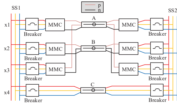
Fig. 5: Schematic for proposed topology 1.
