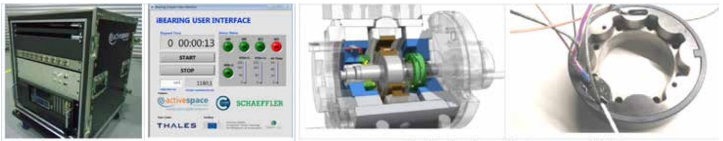
The iBearing mock-up used for proof-of-concept validation.
