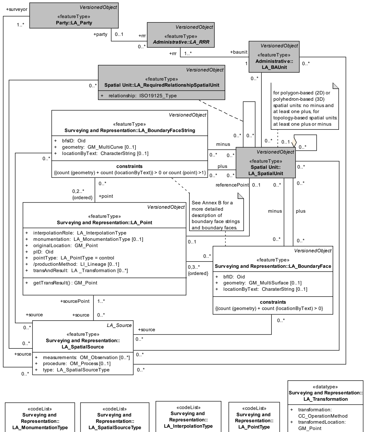
Figure 3 - Content of Surveying and Representation Subpackage with associations to other (basic) classes (ISO, 2012)
