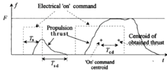
Figure 3. Thrust pulse in time domain (from [24])
