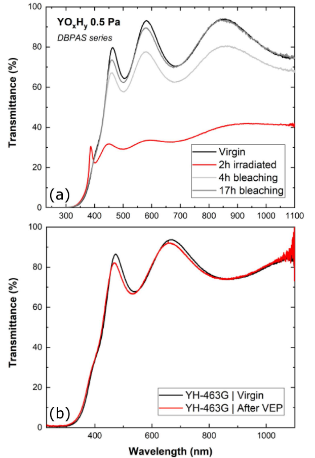
Fig. 1. (a) Optical transmittance spectrum of an \text{YO}_x\text{H}_y sample with a thickness of 385 nm deposited at 0.5 Pa in (i) the as-deposited virgin state and (ii) the state after 2 h of UV-illumination and (iii) after bleaching for 4 h and 17 h. The peak at 385 nm under UV illumination is caused by stray light of the LED light source. (b) Optical transmittance spectrum of the \text{YO}_x\text{H}_y sample with a thickness of 330 nm deposited at 0.5 Pa in (i) the as-deposited virgin state (black line) and (ii) the state after 2 h of UV-illumination and 3 days of bleaching in vacuum in situ during the PAS experiment (red line).
