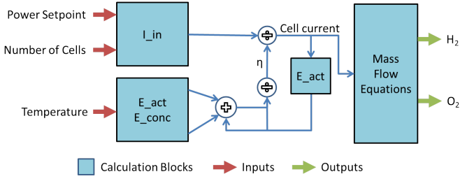
Fig. 1: electrolyzer Model
