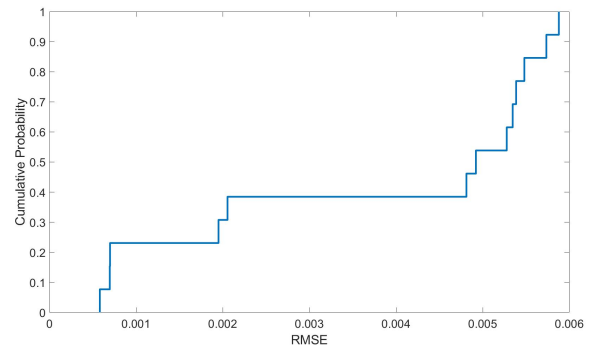
Fig. 9: CDF plot of RMSE ( L_2 ) error
