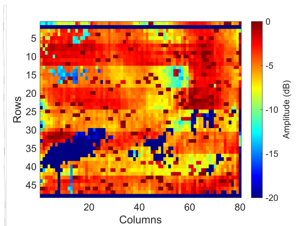
Fig. 4. Relative peak pressure of all transducer elements (corrected for the hydrophone directivity).
