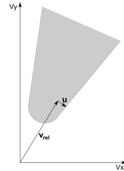
Figure 2. Trimmed velocity obstacle in relative velocity ( \mathbf{v}_{rel} ) space, with minimum velocity change solution ( \mathbf{u} ).
