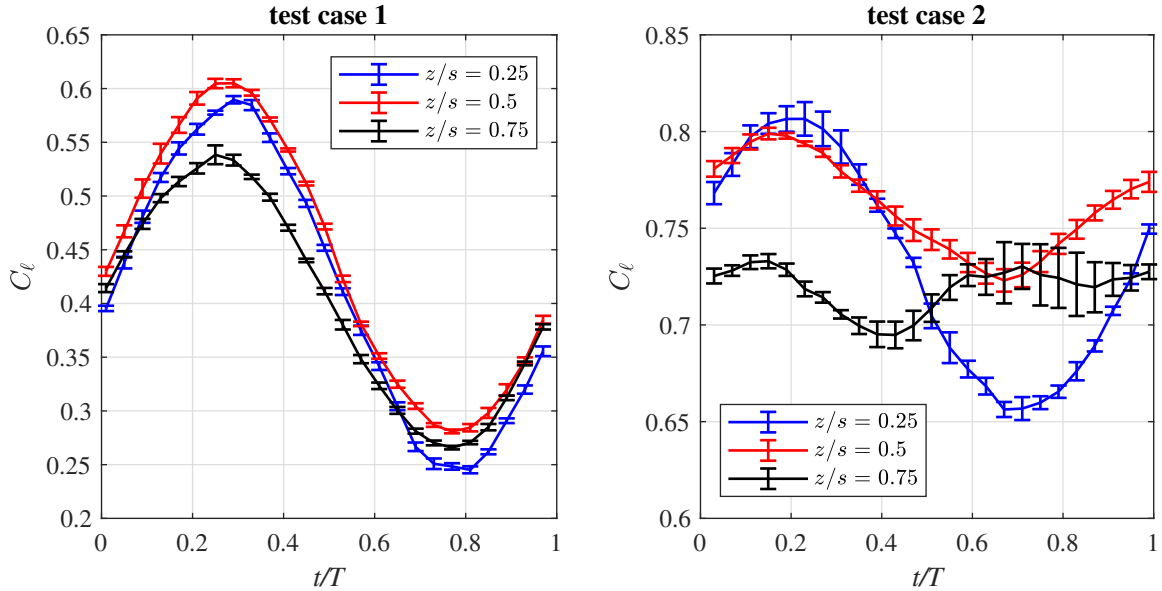
Figure 17: Sectional lift over the period at three different spanwise locations
