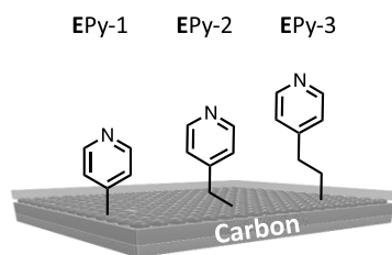
Figure 1. Schematic of case 1: Homogeneous pyridine molecular catalysts with glassy carbon electrodes (GCE) (Py-1, Py-2, and Py-3); case 2: homogeneous pyridine molecular catalysts with silver electrode catalysts (Ag-Py-1, Ag-Py-2, and Ag-Py-3); case 3: heterogeneous electrografted pyridine catalysts onto glassy carbon electrodes (EPy-1, EPy-2, EPy-3); and case 4: heterogeneous electrografted pyridine catalysts onto silver electrodes (Ag-EPy-1, Ag-EPy-2, and Ag-EPy-3).
