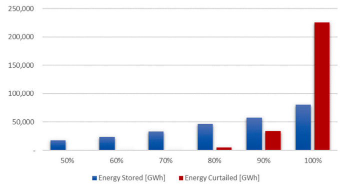
Fig. 9. Energy balance metrics under different decarbonisation objectives.
