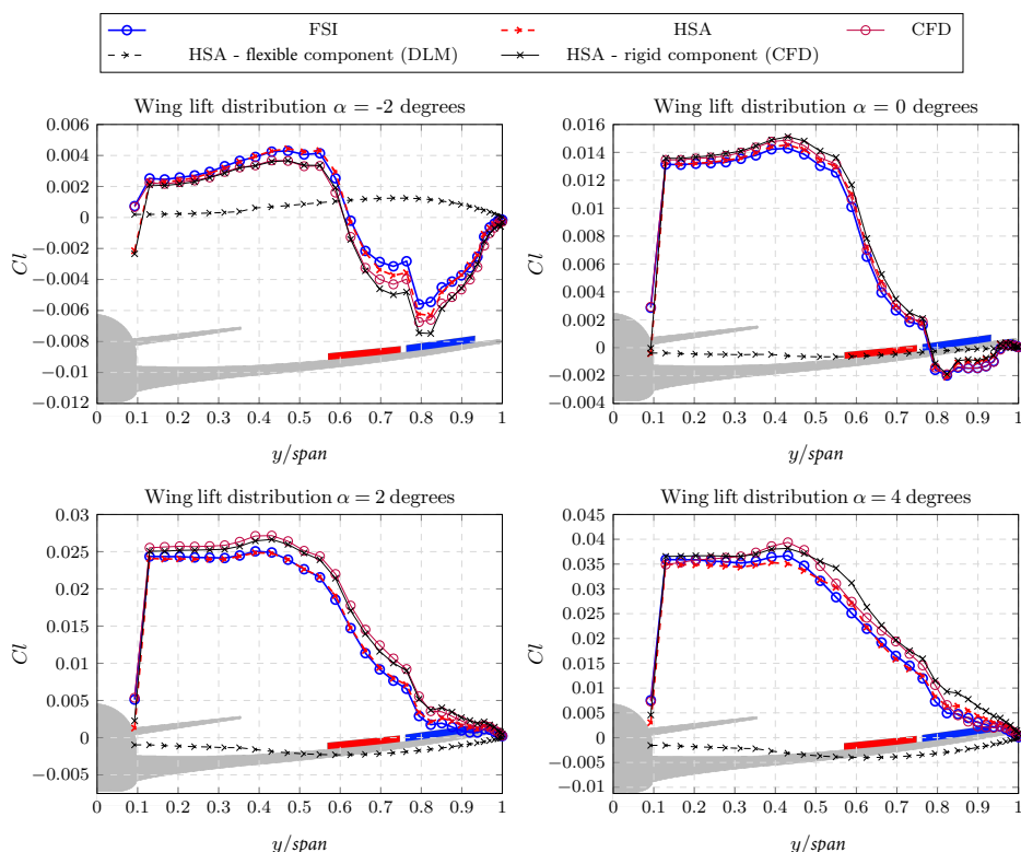
Figure 4.18: Lift distribution span-wise for various angles of attack with the aileron and spoiler deployed obtained with the FSI, CFD and HSA methods for the stiffer wing model at 11,100Pa Mach 0.85.
