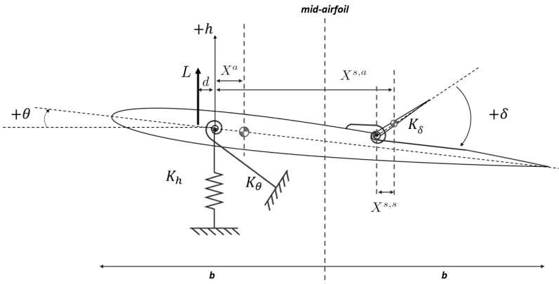
Figure 2.1: Overview of the aeroelastic system with three degrees of freedom: airfoil pitch, plunge and spoiler deflection.
