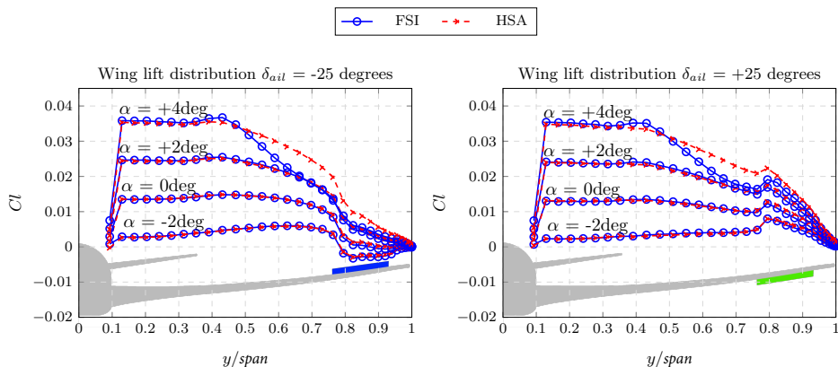
Figure 4.15: Lift distribution span-wise for various angles of attack with the aileron deployed. This is obtained with the FSI and HSA and methods for the wing model A at 11,100Pa Mach 0.85.
