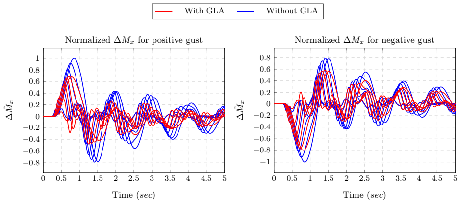
Figure 6.14: Incremental root bending for all gust cases with and without the GLA. The GLA uses the aileron at a deflection rate of 60deg/sec.
