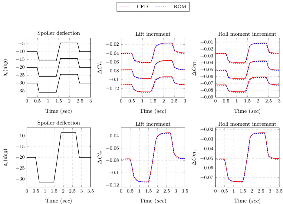
Figure 5.5: Time dependent visualization of the lift and roll moment increment coefficients for various spoiler dynamic deflections.
