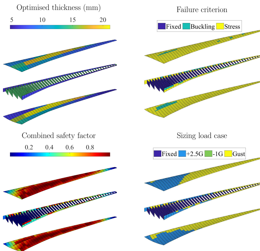
Figure 6.10: Results with no MLA and no GLA.
