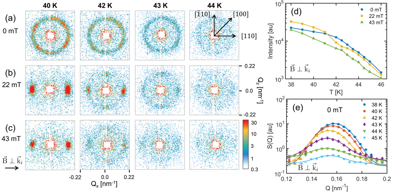
FIG. 2. SANS results obtained at LARMOR by applying the magnetic field perpendicular to the incident neutron beam ( \vec{B} \perp \vec{k}_i ). Characteristic patterns are shown for B = (a) 0, (b) 22, and (c) 43 mT. (d) The temperature dependence of the total scattered intensity for selected magnetic fields. (e) S(Q) in arbitrary units, deduced by radially averaging the scattered intensity at a magnetic field of 0 mT, for the temperatures indicated. The solid lines indicate the best fits of Eq. (1) to the data.
