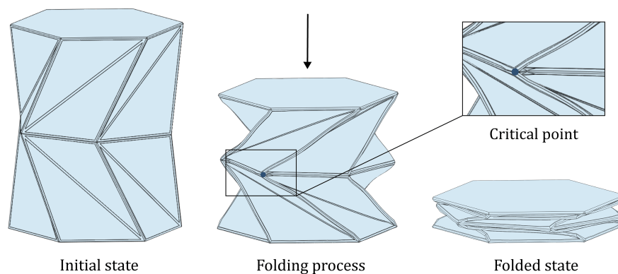
Fig. 11 Folding process.
