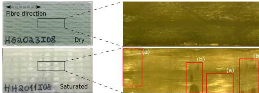
Figure 11: In-plane microscopic comparison of dry and saturated specimens, with (a) debonding in the 0^\circ direction and (b) debonding in the 90^\circ stabilization roving.
