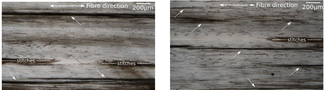
Figure 12: Through-thickness micrographs of a saturated specimen with arrows indicating debonded regions.
