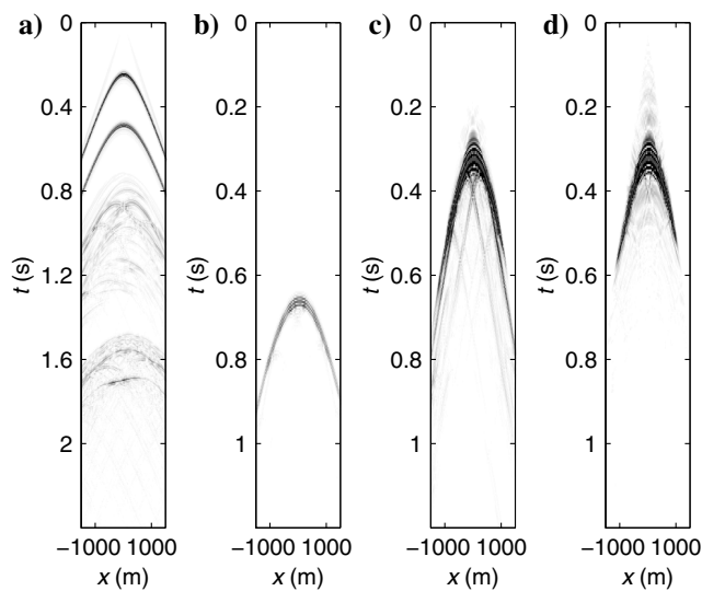
Figure 3. (a) Reflection response with a source at x = 0 at the acquisition boundary \mathcal{S}_a and receivers at the same boundary. (b) Direct wavefield with a source at x = 0 at \mathcal{S}_a and receivers at \partial\mathcal{V}_j , computed by time gating the transmitted wavefield in the physical medium. (c) Transmission response from above with a source at x = 0 at \partial\mathcal{V}_i and receivers at \partial\mathcal{V}_j , computed in the reference medium. (d) Similar transmission response, obtained by target-enclosed redatuming of the Green's functions (i.e., inversion of equation 15). All figures have been normalized with respect to their maximum value. Panels (c) and (d) have been enhanced by a factor 20 and are clipped at 5% of the maximum value to emphasize weak arrivals.
