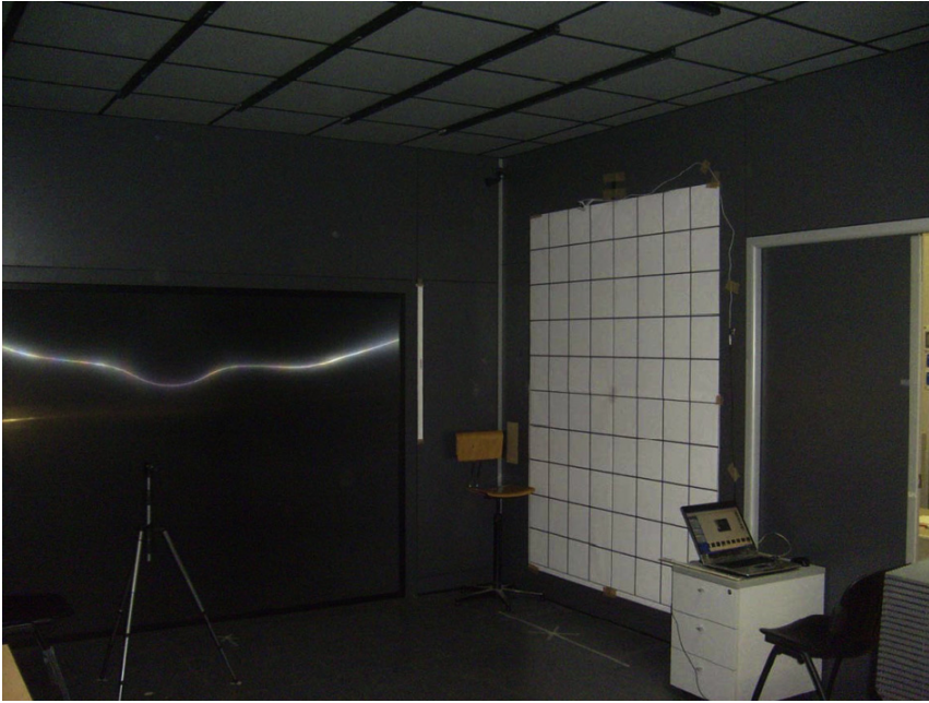
Fig. 3.1: VR-Lab set-up: graduated paper sheet and acquisition devices
