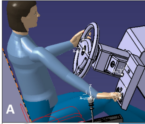
Fig. 8.17: DELMIA® simulation
