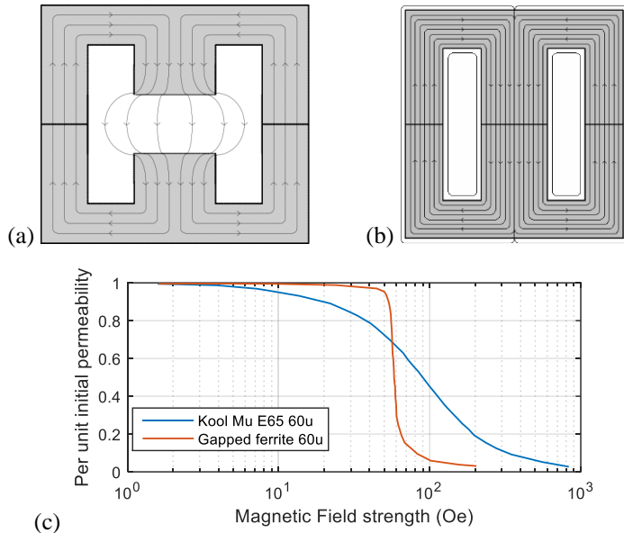
Fig. C.1. Path of flux lines through a (a) gapped ferrite core and (b) a powdered iron core. (c) Variation of permeability of core as a function of magnetic field strength for a KoolMu powdered iron core and gapped ferrite core, both of which have an initial permeability of \mu_r=60 (bottom) [19]
