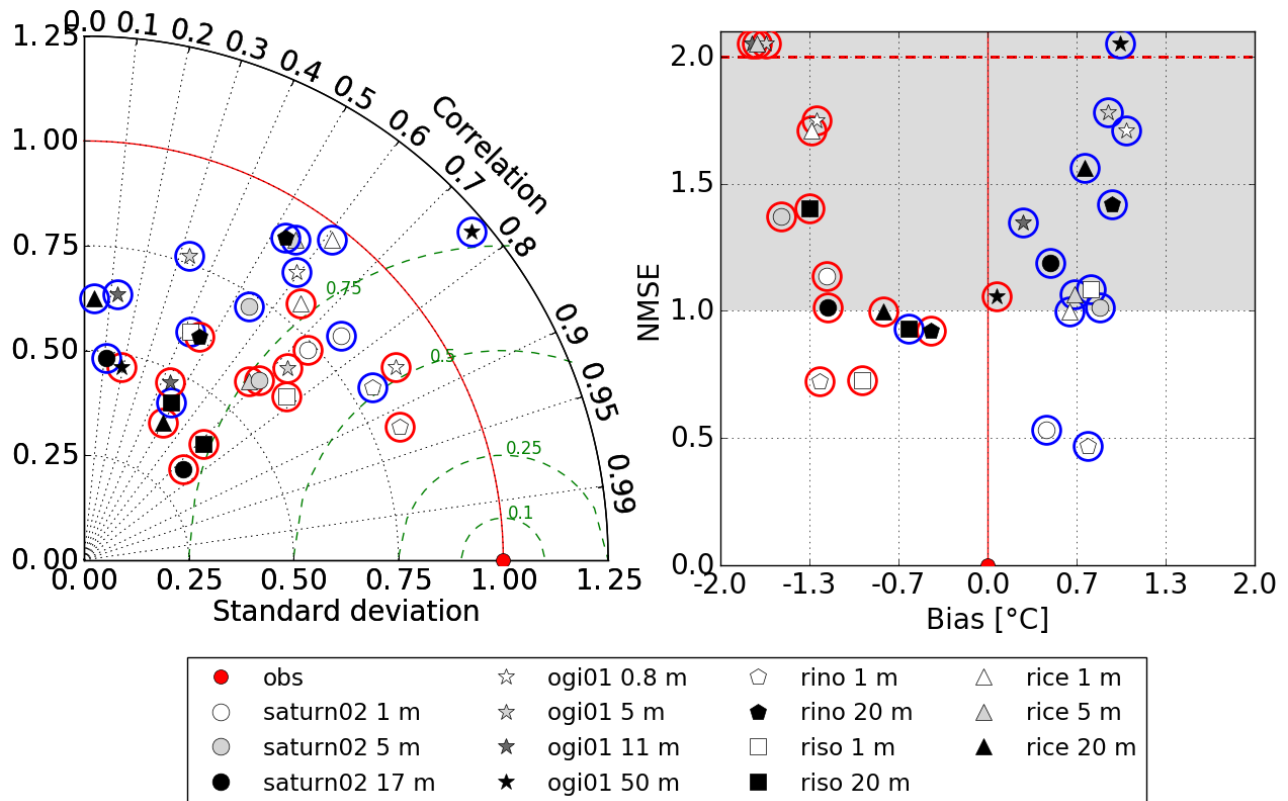
Figure 8: Normalized Taylor diagram (left) and NMSE versus bias (right) for SLIM 3D (red circles) and SELFE (blue circles) models outputs on the shelf for temperature. The grayscale of the markers indicate the depth: white is shallower, dark is deeper. In the Taylor diagram, normalized standard deviation is on the radial axis; correlation coefficient is on the angular axis; green dashed lines indicate NCRMSE. On the right panel, NMSE larger than 2 are placed just above the red dashed line irrespective of their values (see Table 2 for exact values). SLIM 3D skill is in general better than SELFE in terms of correlations and NCRMSE, but slightly worse in terms of biases.
