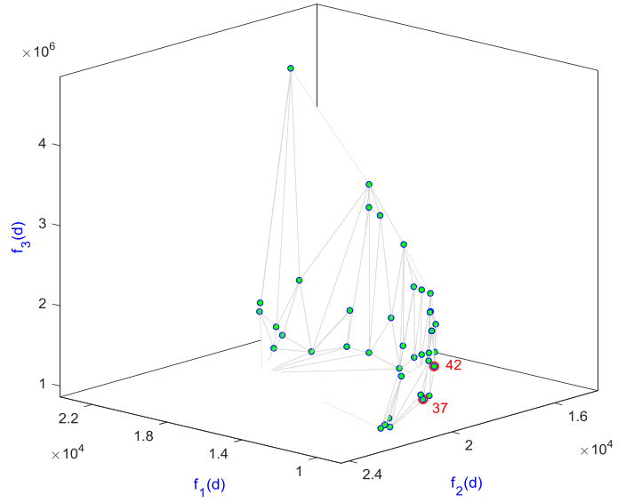
Fig. 5. Pareto fronts obtained by the second problem.
