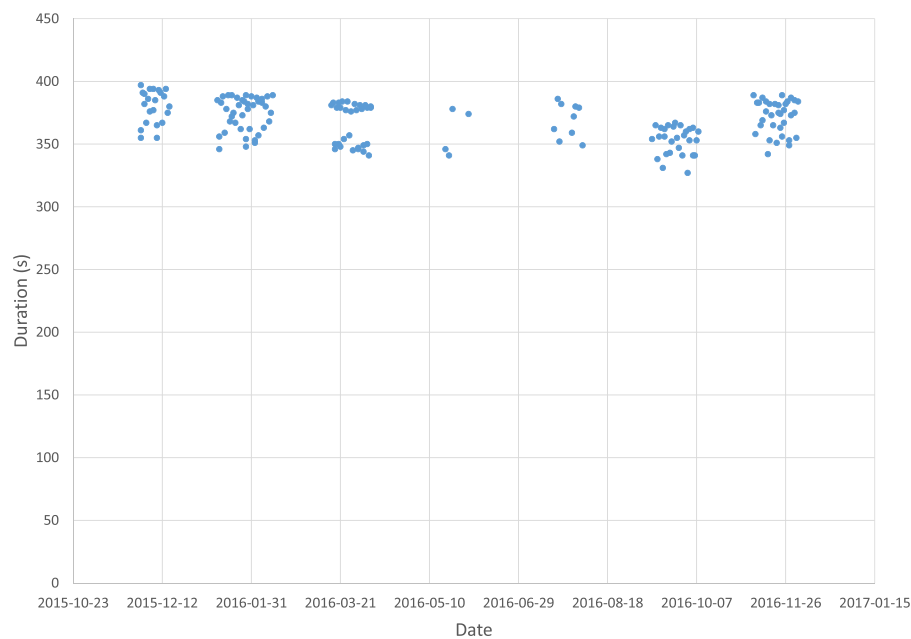
Figure 5 12 Month Pass Analysis of the ISS over MLRO. The distribution of durations for suitable passes over the OGS is shown. Passes were restricted to orbits rising at least 30^\circ above the horizon and occurring in eclipse. The pass duration is counted as the time spent above 10^\circ above the horizon though the actual time available for quantum transmission will be less than this.
