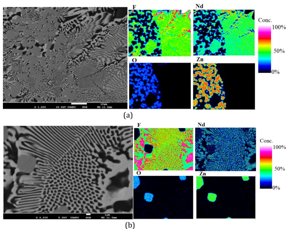
Figure 4.6– EPMA mapping images of \text{LiF-Nd}_2\text{O}_3\text{-ZnF}_2 sample after fluorination treatment, (a) analysed at 15 kV and (b) at 5 kV.
