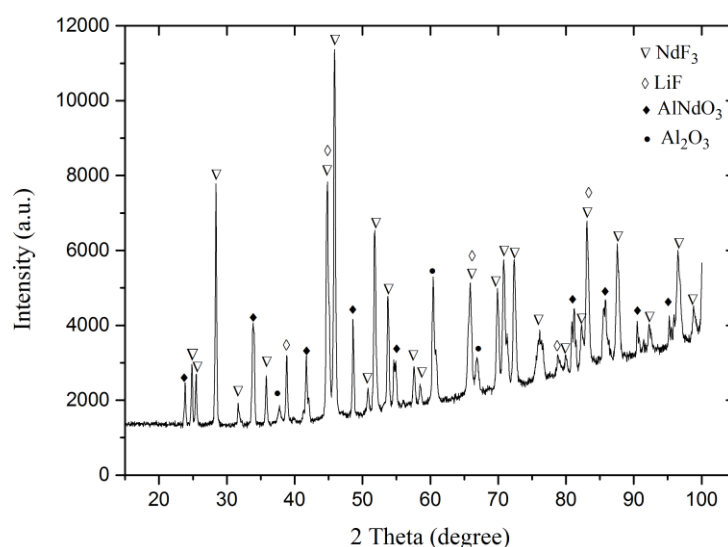
Figure 4.2– XRD pattern of LiF- \text{Nd}_2\text{O}_3 - \text{AlF}_3 sample after fluorination treatment with identified phases.
