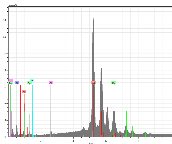
Figure 2.9– EDS pattern of Dy-Nd deposit on graphite cathode in LiCl-KCl-NaCl molten salt at 800°C.
