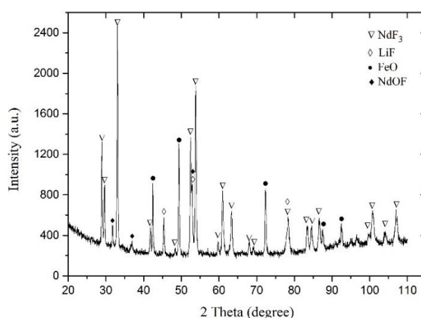
Figure 4.8 – XRD pattern of LiF-Nd 2 O 3 -FeF 3 sample after fluorination treatment with identified phases
