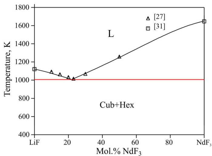
Figure 6.3– Calculated LiF-NdF 3 phase diagram and comparison with the experimental data from [27, 31].
