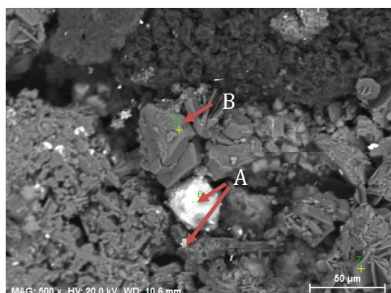
Figure 2.8– SEM image of cathode deposition after electrolysis of magnet, using \text{AlCl}_3 as flux, at V=3.4 V and T=800^\circ\text{C} during 6 hours. A is the metallic phase (Dy-Nd), B is the oxide phase.
