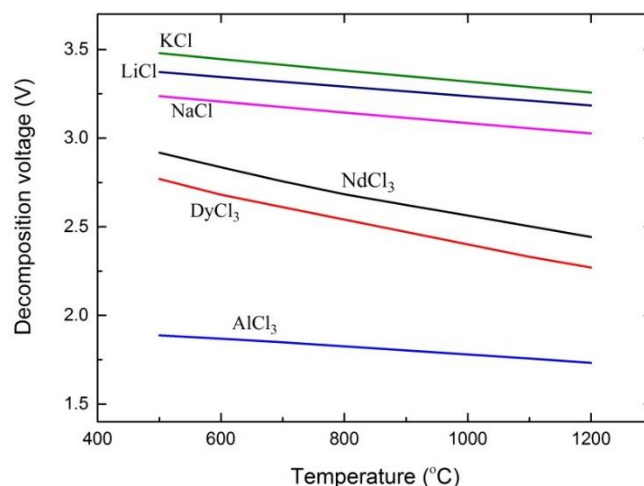
Figure 2.1– Calculated standard decomposition voltage as a function of temperature for the chlorides formed in LiCl–KCl–NaCl–AlCl 3 molten salt bath.
