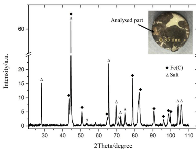
Figure 5.11– XRD result of the part of the salt under the Fe anode in \text{LiF-NdF}_3 salt bath.
