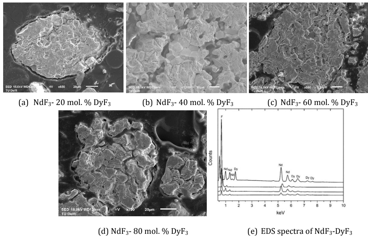
Figure 6.2– BSE image and EDS spectra of selected compositions.
