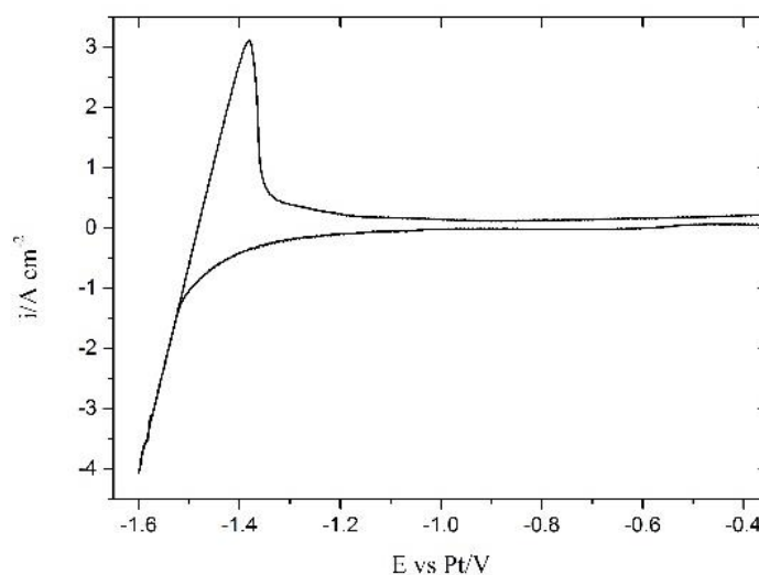
Figure 5.9– Cyclic voltammograms of \text{LiF-Nd}_2\text{O}_3 on a Mo electrode ( \phi\ 2\text{ mm} \times 40\text{ mm} ) at 950^\circ\text{C} , counter electrode: glassy carbon, reference electrode: Pt wire, scan rate: 100\text{ mVs}^{-1}
