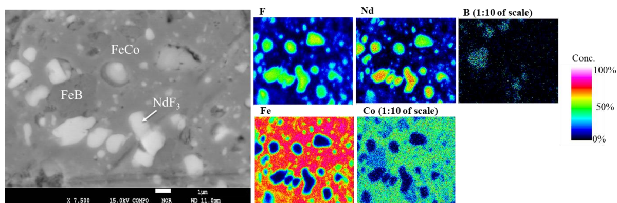
Figure 3.9– EPMA mapping of the LiF-NdFeB-FeF 3 sample after fluorination treatment.
