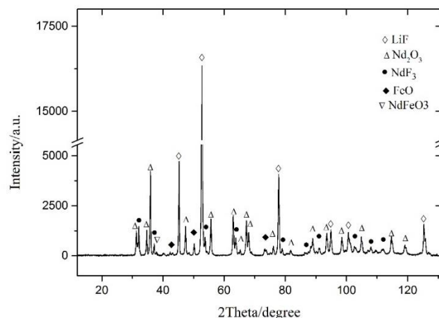
Figure 5.15– XRD result of the sample of \text{LiF-Nd}_2\text{O}_3\text{-FeF}_3 electrolyte after electrolysis with iron anode and Mo cathode.
