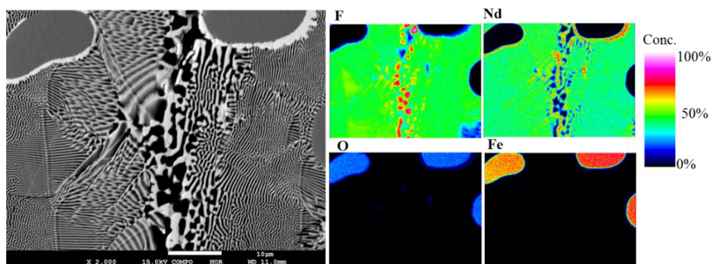
Figure 4.9– EPMA mapping of LiF- \text{Nd}_2\text{O}_3 - \text{FeF}_3 sample after fluorination treatment showing the presence of \text{NdF}_3 and FeO.
