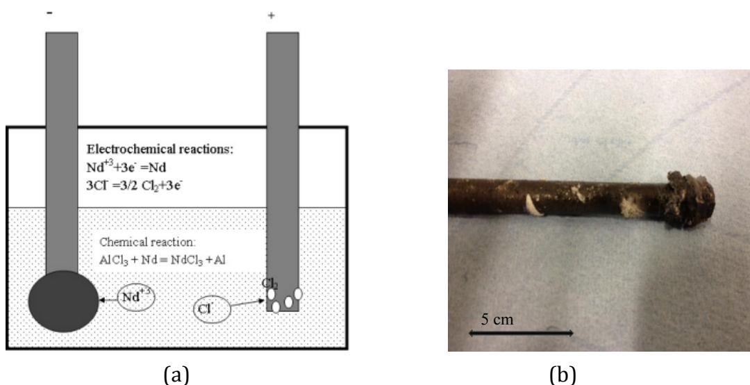
Figure 2.7– (a) Schematic diagram of the set-up (b) Image taken from graphite cathode after electrolysis at 800°C for 6 hours in argon atmosphere.
