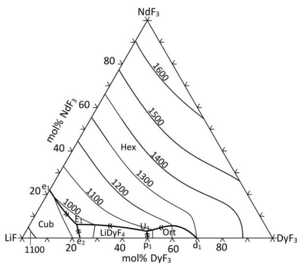
Figure 6.6– Calculated liquidus projection for the LiF-DyF 3 -NdF 3 system (temperature in K).
