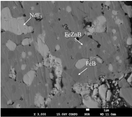
Figure 3.7– BSE image of the LiF-NdFeB-ZnF 2 sample in at% after fluorination treatment showing the presence of NdF 3 , FeB and FeZnB.
