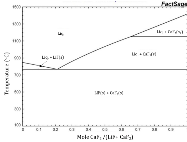
Figure 2.3– LiF-CaF 2 phase diagram from FactSage software package [15]
