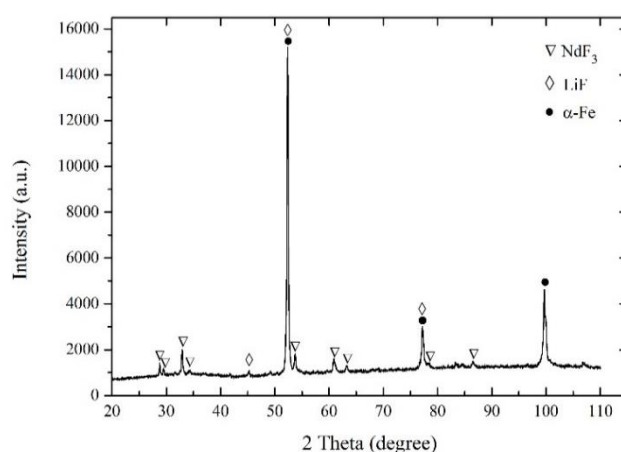
Figure 3.8– XRD pattern with phase identification of the LiF-NdFeB-FeF 3 sample after fluorination treatment.
