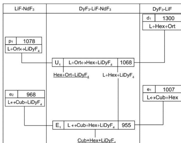
Figure 6.7– Reaction scheme for the DyF 3 -LiF-NdF 3 system.
