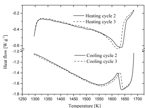
(a) NdF 3 -20 mol% DyF 3
