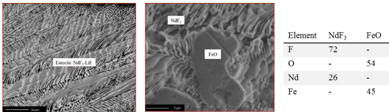
Figure 4.10– BSE image and EPMA quantification result of LiF- \text{Nd}_2\text{O}_3 - \text{FeF}_3 sample in at% after fluorination treatment showing the presence of \text{NdF}_3 and FeO.
