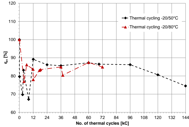
Figure 14: Combined ILSS graph for heated GLARE 5-2/1-0.3 specimens thermal cycled between -20 to 50 °C and -20 to 80 °C in comparison with the reference (cf. Table 1).
