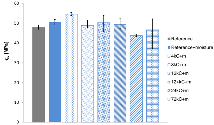
Figure 10: Absolute ILSS values for heated GLARE 5-2/1-0.3 specimens HGL1M to HGL6M thermal cycled between -20 and 80 °C (cf. Table 1).
