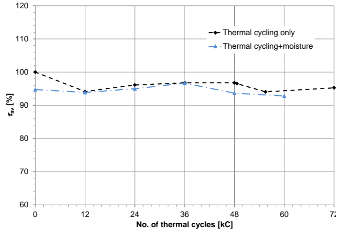
Figure 8: Relative ILSS values for heated glass-fibre epoxy specimens HGE1(M) to HGE6(M) thermal cycled between -25 and 95 °C with and without prior conditioning to 0.3% moisture content (cf. Table 1).
