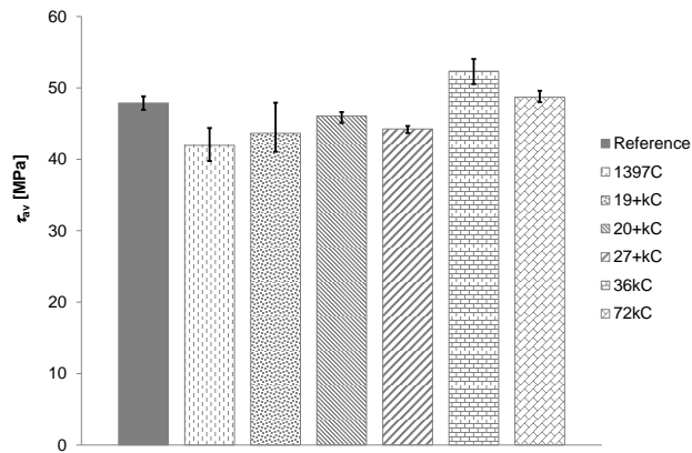
Figure 9: Absolute ILSS values for heated GLARE 5-2/1-0.3 specimens HGL1 to HGL6 thermal cycled between -20 and 80 °C (cf. Table 1).
