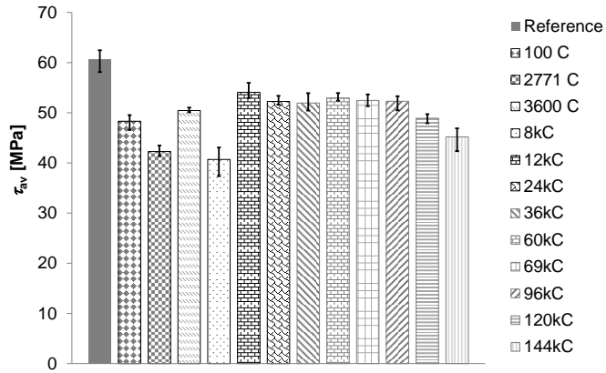
Figure 12: Absolute ILSS values for heated GLARE 5-2/1-0.3 specimens HGL10 to HGL23 thermal cycled between -20 and 50 °C (cf. Table 2).
