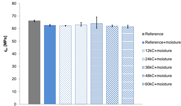
Figure 7: Absolute ILSS values for heated glass-fibre epoxy specimens HGE1M to HGE6M thermal cycled between -25 and 95 °C after conditioning to 0.3% moisture content (cf. Table 1).
