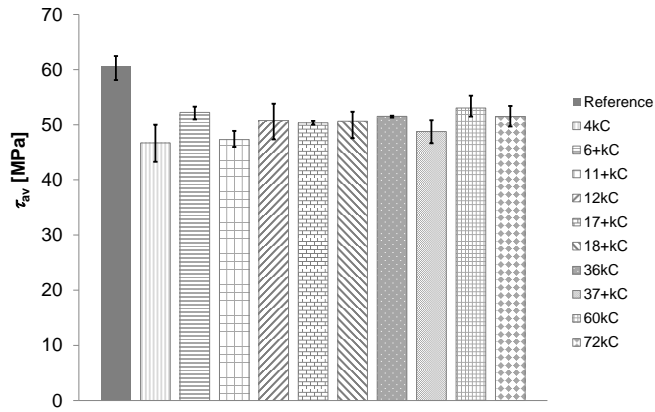
Figure 13: Absolute ILSS values for heated GLARE 5-2/1-0.3 specimens HGL31 to HGL36 thermal cycled between -20 and 80 °C (cf. Table 2).
