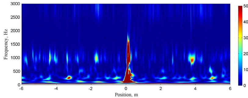
Fig. 5. Scalogram of the ABA signal around a moderate squat located in a track section between Groningen and Assen, The Netherlands.
