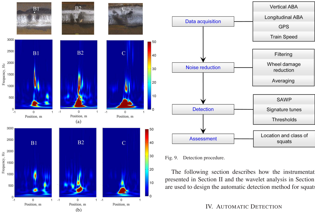
Fig. 8. WPS at typical moderate and severe squats found in The Netherlands. (a) WPS at squats. (b) WPS on the opposite axle.
