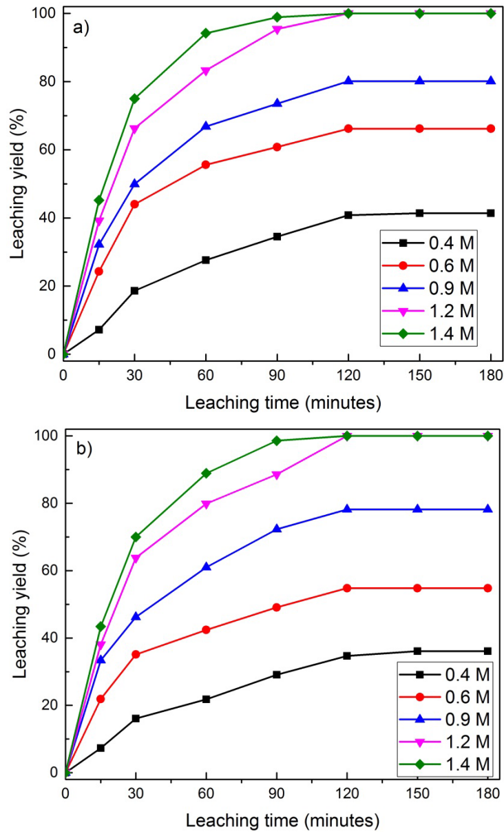
Figure 2.2 Effect of acid concentration on the leaching yield (%) of (a) REEs and (b) iron from NdFeB magnet waste powder (Stirring rate 550 rpm, T = 25^\circ\text{C} , C_{\text{NH}_4\text{Cl}} = 3\text{M} ). Relative standard deviation < 3.6\% .
