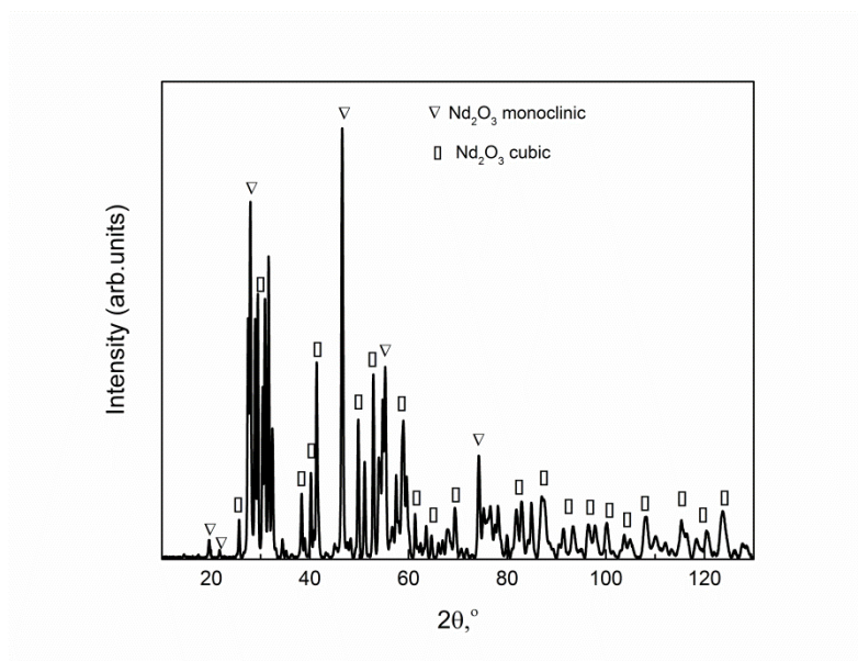
Figure 4.7 XRD pattern of the obtained rare-earth oxide.
