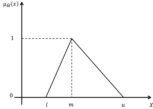
Fig. 4. Schematic of a triangular fuzzy number (Zimmermann 2011).
