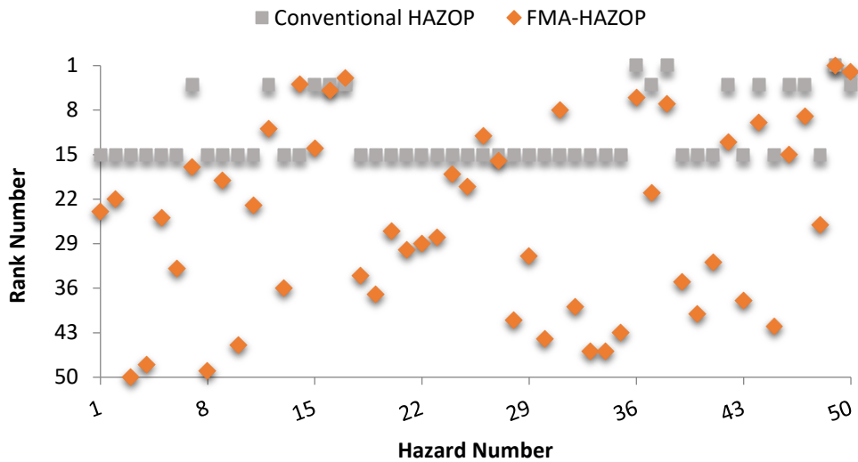
Fig. 7. Hazards ranking in conventional HAZOP and FMA-HAZOP.
