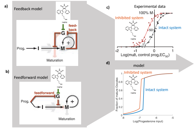
Fig. 2: Inhibition of double-negative GSK - 3\beta feedback loop shifts the dose response of maturation as a function of the progesterone stimulus, making the switch occur at lower level of stimulus. (a) Feedback model block diagram. GSK - 3\beta double negative feedback loop can be disabled by addition of the inhibitor 7AIPM. (b) A plausible feedforward model involving GSK - 3\beta . (c) Fraction of mature Oocytes as a function of progesterone stimulus determined experimentally in wild type and following inhibition of GSK - 3\beta with 7AIPM to disable the double negative GSK - 3\beta feedback loop. (d) Fraction of mature Oocytes as a function of stimulus (progesterone) for models following inhibition of G . Both feedback and feedforward loop architectures can produce a similar shift of the dose response observed in the data. Results adapted from [63].
