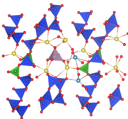
Figure 5: Computed local structure of a silicate glass containing Mo, from Konstantinou (2017)
