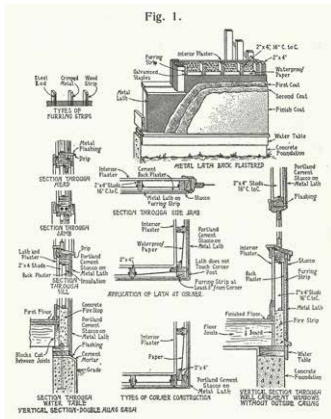
FIG. 5.7 An American system for light façade construction was copied with slight modification for the Sanatorium 'Zonnestraal' buildings – the wooden studs were replaced by steel ones. Structural engineer Wiebenga had already proposed this alteration when he described the original system in 'Gewapend Beton' in 1926 / source unknown
