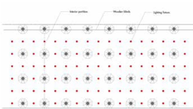
FIG. 5.18 Van Nelle Factory: scheme of the original distribution of service systems at the ceilings of the factory halls / Claessens Erdmann Architects
