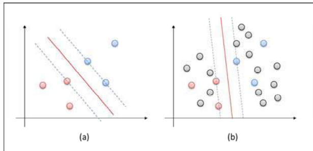
Figure 4. Difference between SVMs and S3VMs; a) SVM decision boundary, b) S3VM decision boundary.
