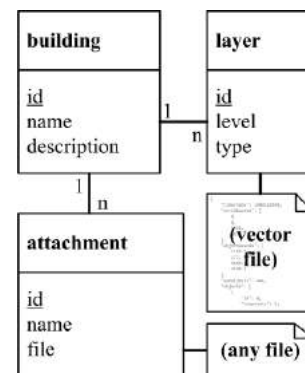
Figure 2. Database representation and linked files.
