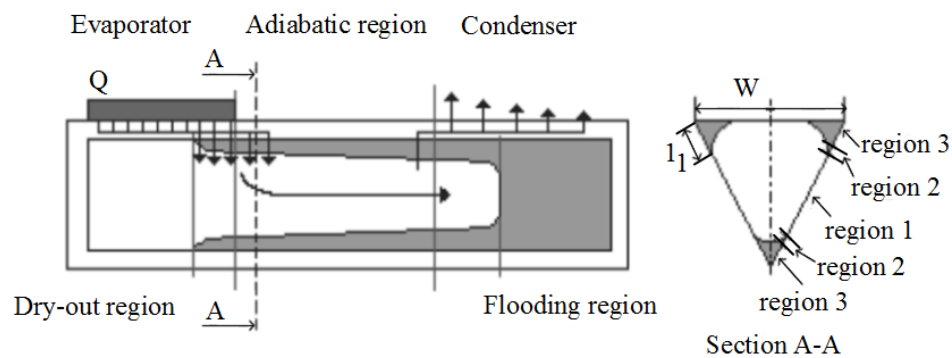
Figure 4. Micro heat pipe with triangular capillary microchannels [13, 30].
