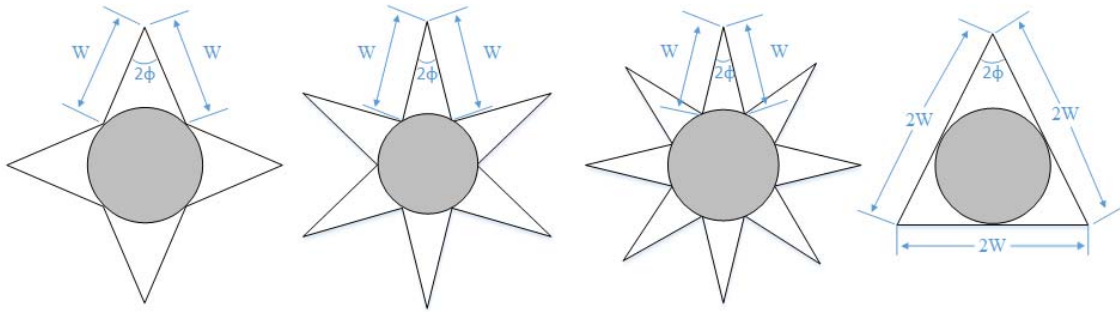
Figure 5. Geometry of different cross-sectional shape of micro-heat pipes [43].
