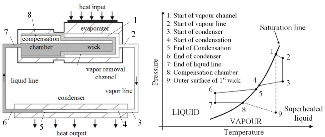
Figure 7. Geometry of an LHP and T diagram for LHP steady-state operation (capillary controlled mode) [51, 52, 55, 56].
