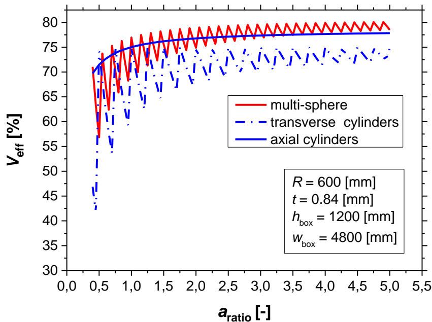
Fig. 5-19: Volumetric efficiency of i) multi-spherical, and cylindrical pressure vessels in ii) axial and iii) transverse packaging for a box with variable a_{\text{ratio}} at ambient conditions.
