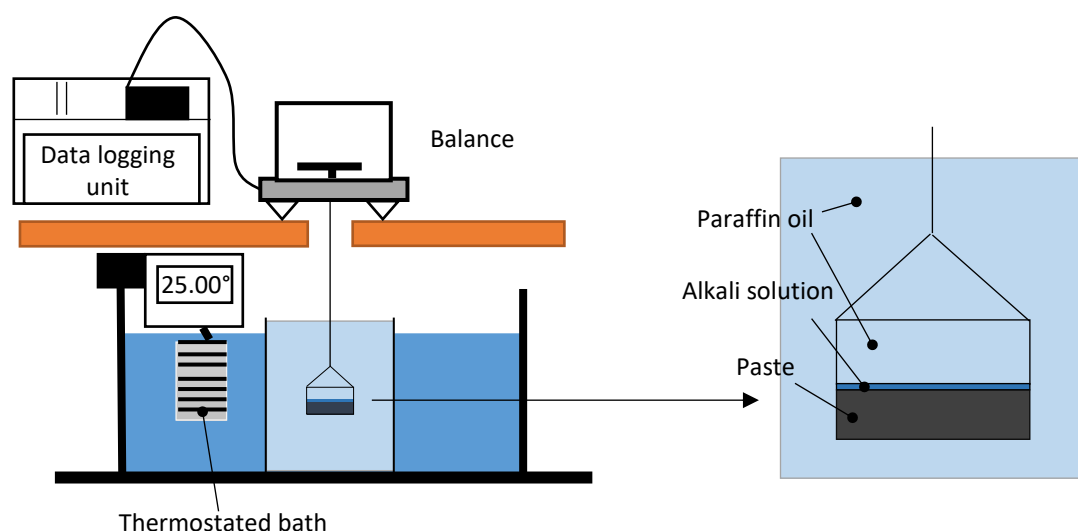
Fig.1 Schematic of devices for chemical shrinkage measurement, after [21].
