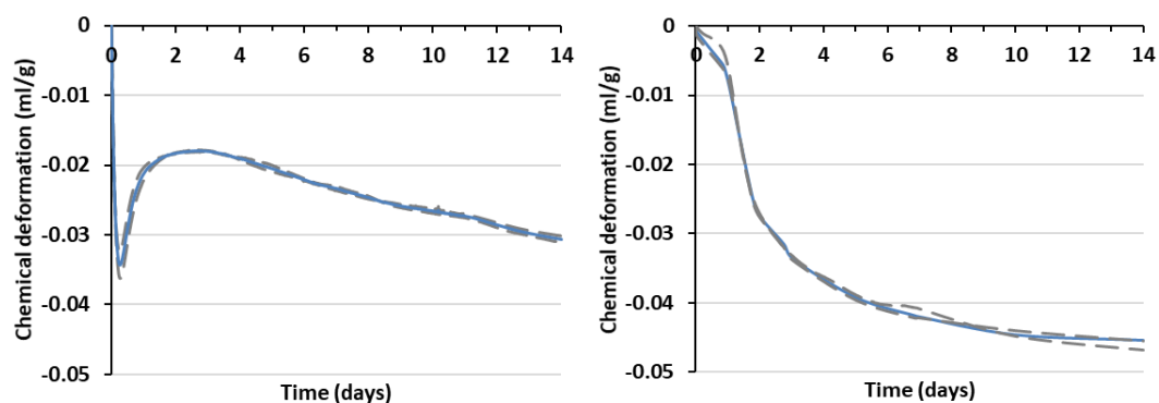
Fig. 2. Chemical deformation of (a) MKG paste, and (b) OPC paste. A representative curve is shown in solid line while the other two curves are shown in grey dashed lines. The curves indicate a good repeatability of the measurement.
