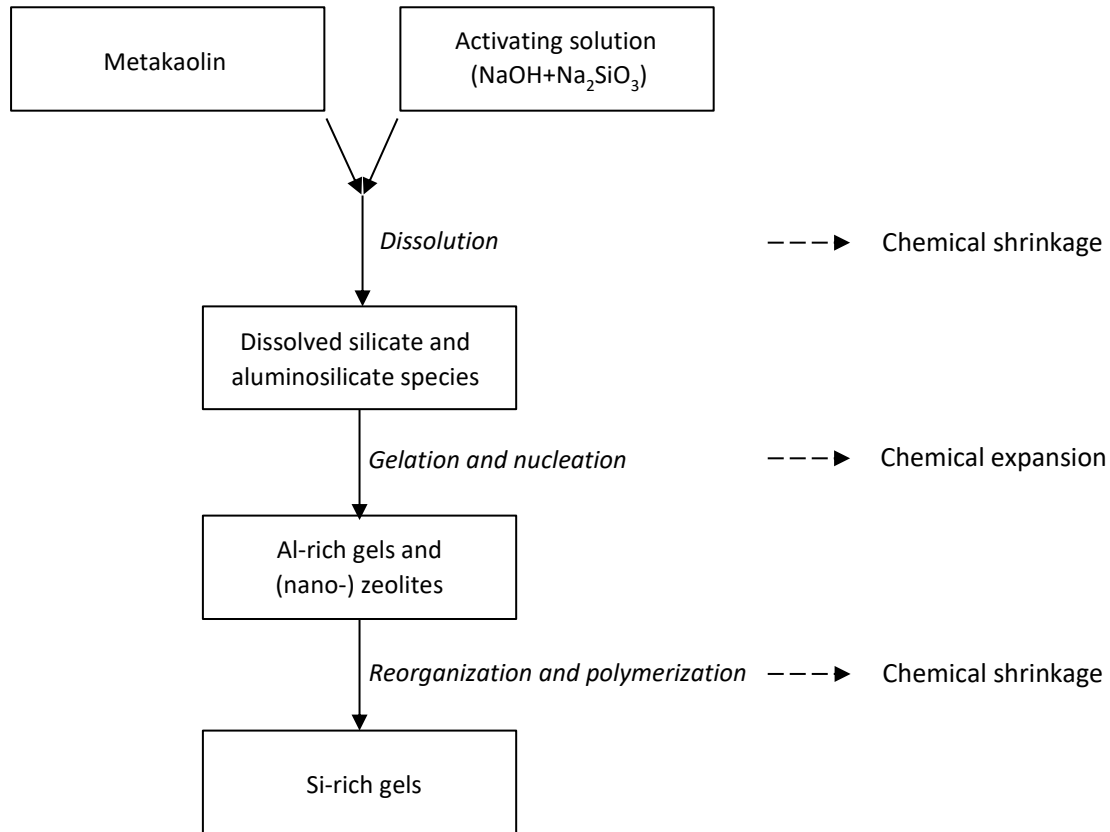
Fig.10. Reaction processes and chemical deformations of geopolymerization.
