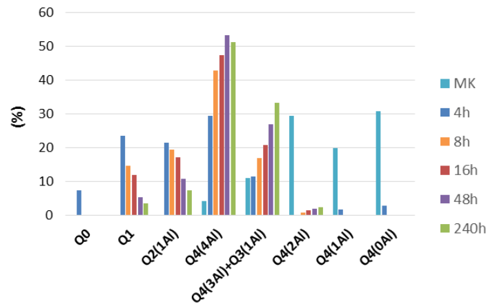
Fig.7. Normalized summary of Qn(mAl) Si coordination environments within MK and MKG pastes identified in the deconvoluted ^{29}\text{Si} NMR spectra.
