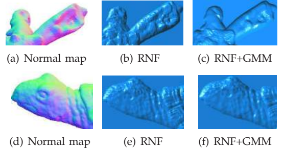
Fig. 7. Using RNF plus GMM can prevent the residual normals N_B^r induced from the base surface.
