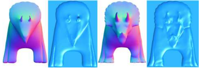
Fig. 10. Rendering the base surface normal field on the original mesh (the third one) can better preserve the overall shape of an object when generating the corresponding bas-relief (the last one). If we really update a mesh to match the base normal field to obtain a base mesh [12] and render it (the first one), the shape distortion would happen when performing bas-relief modeling (the second one)
