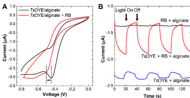
Figure 2. (A) Cyclic voltammetric diagrams of TsOYE in alginate film in the presence and the absence of RB. (B) Photocurrent response of TsOYE in alginate film at an applied potential of -0.6 V (vs Ag/AgCl, 3 M NaCl). A MOPS buffer (50 mM, pH 7.5) was used with Ag/AgCl and Pt as a reference electrode and a counter electrode, respectively.
