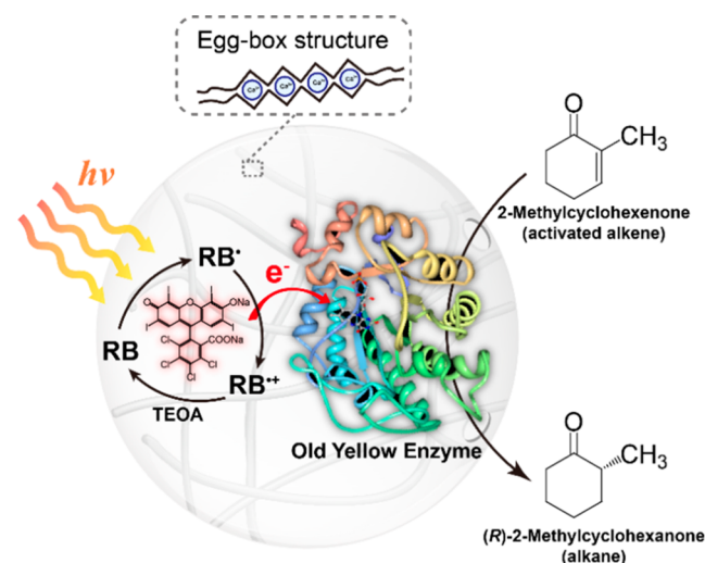
Scheme 1. Schematic Illustration of a RB and TsOYE Encapsulated Alginate Capsule for OYE Photobiocatalysis a
