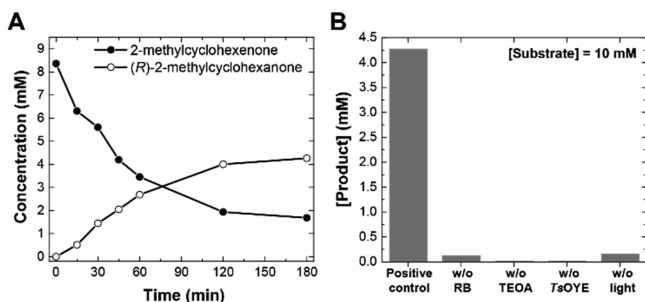
Figure 3. (A) Conversion of 2-methylcyclohexenone to ( R )-2-methylcyclohexanone by RB- TsOYE /alginate beads. Reaction conditions: [2\text{-methylcyclohexenone}] = 10 \text{ mM} , [TsOYE]_{\text{in alginate}} = 21 \mu\text{M} , [RB]_{\text{in alginate}} = 140 \mu\text{M} , 200 mM TEOA buffer (pH 7.5), reaction temperature = 30^\circ\text{C} , white LED illumination. (B) Control experiments about the effect of each reaction component. A 50 mM MOPS buffer (pH 7.5) was used for the without-TEOA case.
