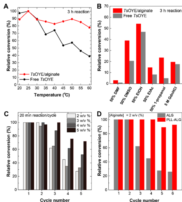
Figure 5. Series of stability tests for RB-TsOYE/alginate beads in terms of relative conversion upon (A) temperature change and (B) solvent addition. Series of recycle tests for RB-TsOYE/alginate beads by (C) varying alginate concentration and (D) coating a poly-L-lysine layer. [Substrate] = 10 mM, [TEOA] = 200 mM, reaction temperature = 30 °C.
