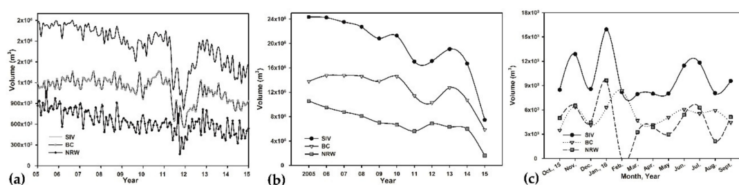
Figure 3. Fluctuation in the NRW volume according to changes in SIV: (a) monthly basis for the full-scale system; (b) annual basis for the full-scale system; (c) monthly basis for DMA-1 in Hadda Zone, Sana’a.
