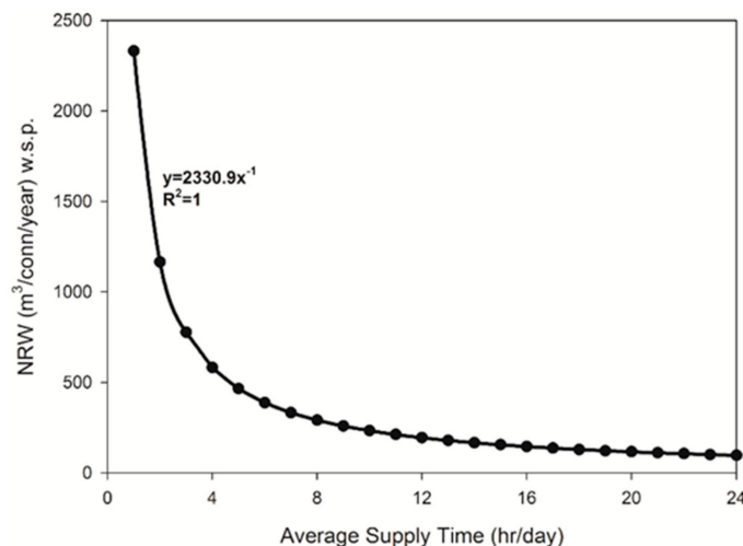
Figure 4. Sensitivity of the normalised NRW volume (w.s.p.) to the average supply time in Sana’a water distribution system.
