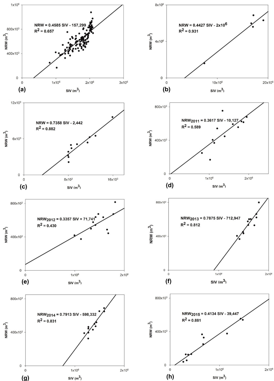
Figure 5. NRW–SIV regression equations; (a) monthly volumes for 2005–2015; (b) annual volumes for 2011–2015; (c) monthly volumes for a DMA in Sana'a; and (d)–(h) monthly volumes for 2011, 2012, 2013, 2014 and 2015, respectively.
