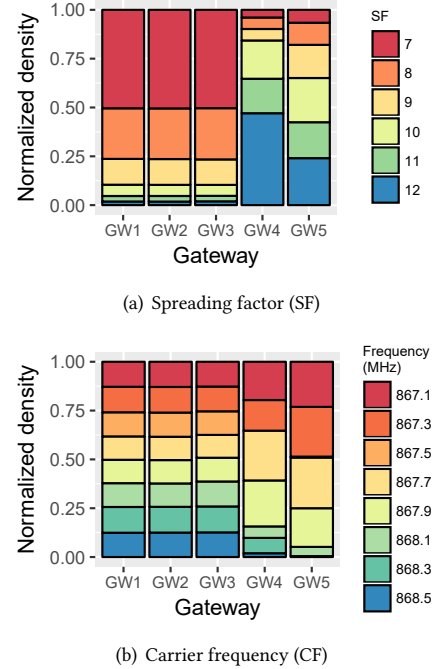
Figure 6: Histogram of SF and CF of KISS LoRa devices obtained from the received frames per gateway.
